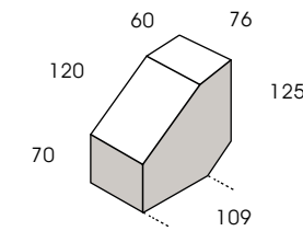
CB SILL
